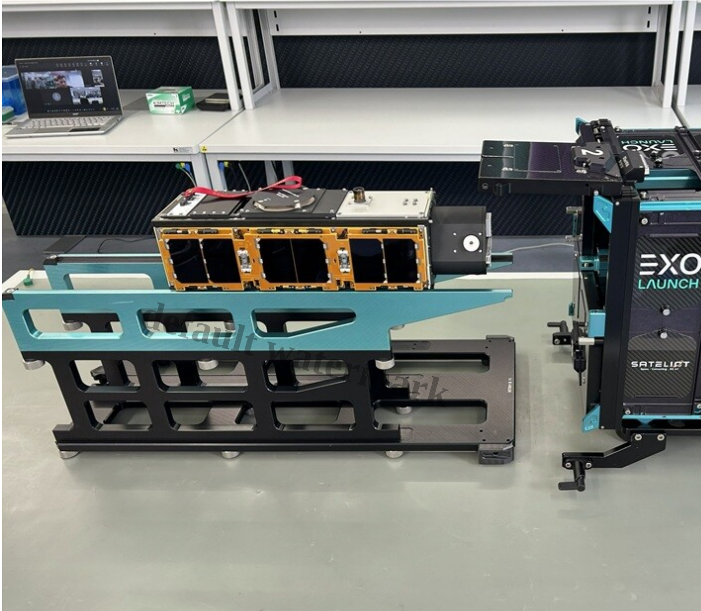
CRIMSON-1 being integrated with the Exolaunch EXOpod Nova system. Photo: NTU Singapore
